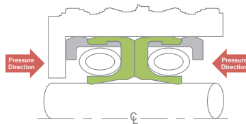
Bi-directional Seal Medium-speed, Low-pressure
