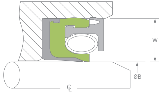
Series LKS
