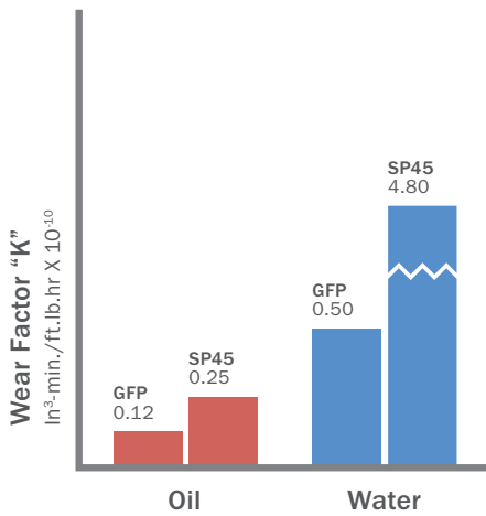
Wear Rate at 100,000 PV Low speed (100 fpm) – High pressure (1000 psi)
