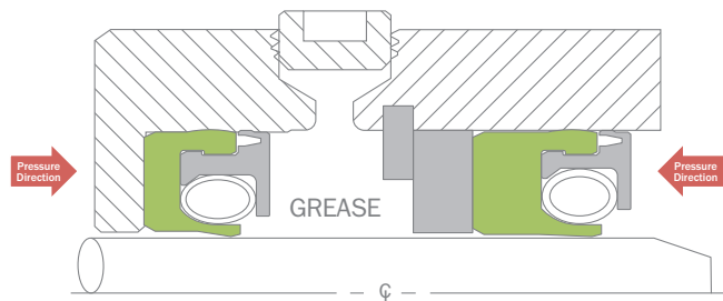
Seal for Medium-speed Low Differential Pressures
