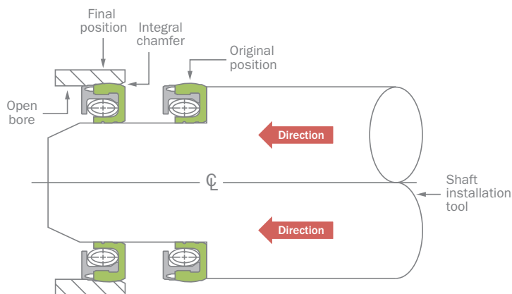
Assembly in open bore
