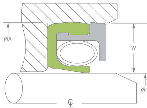
Series KS
