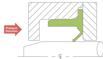
High-speed Flanged Seal
