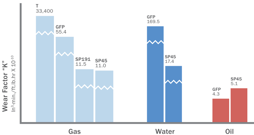
Wear Rate at 20,000 PV Speed (20 fpm) – Pressure (1000 psi)
