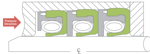
Multi-sealing, Medium-speed, Medium-pressure
