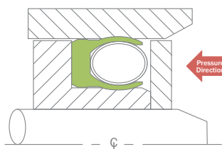
Cryogenic Seal for Low-speed with Ribbon Spring
