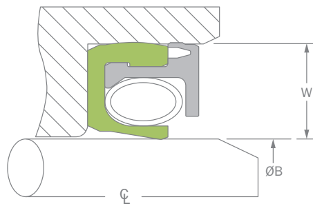
Series KS
