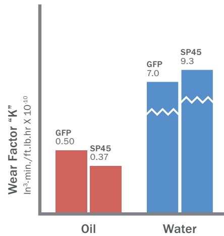
Wear Rate at 100,000 PV High speed (1000 fpm) – Low pressure (100 psi)
