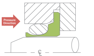
Sealing, Medium-speed, Medium-pressure
