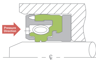
Anti-blowout Seal
