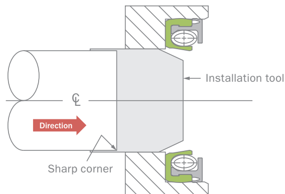
Assembly of shaft from forward direction
