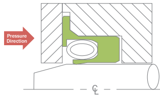
Front-flanged, High-speed, Medium-pressure Seal
