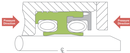
Bi-directional Seal Low-speed, Low-pressure
