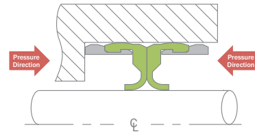
Multi-sealing, High-speed, Low-pressure Seal
