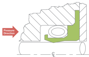
Cryogenic Seal, Medium-speed, Very Low Pressure
