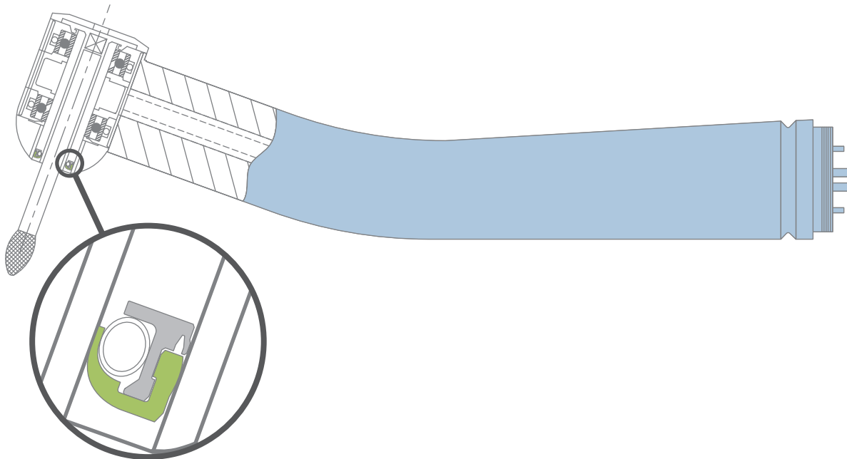
Bal Seal® KTS Series Seal
