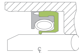
High-speed Seal
