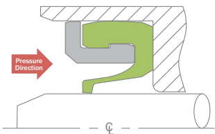
High-speed Seal
