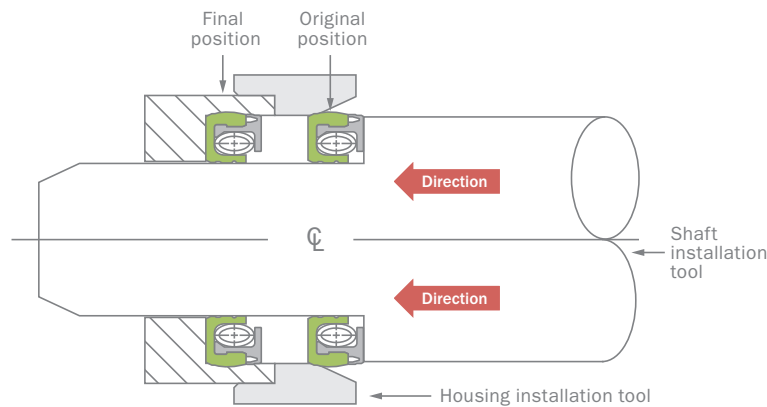
Assembly in gland with sharp entry corner
